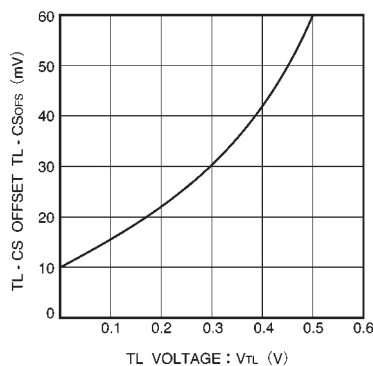
Fig. 21 TL-CS offset vs. VTL voltage
